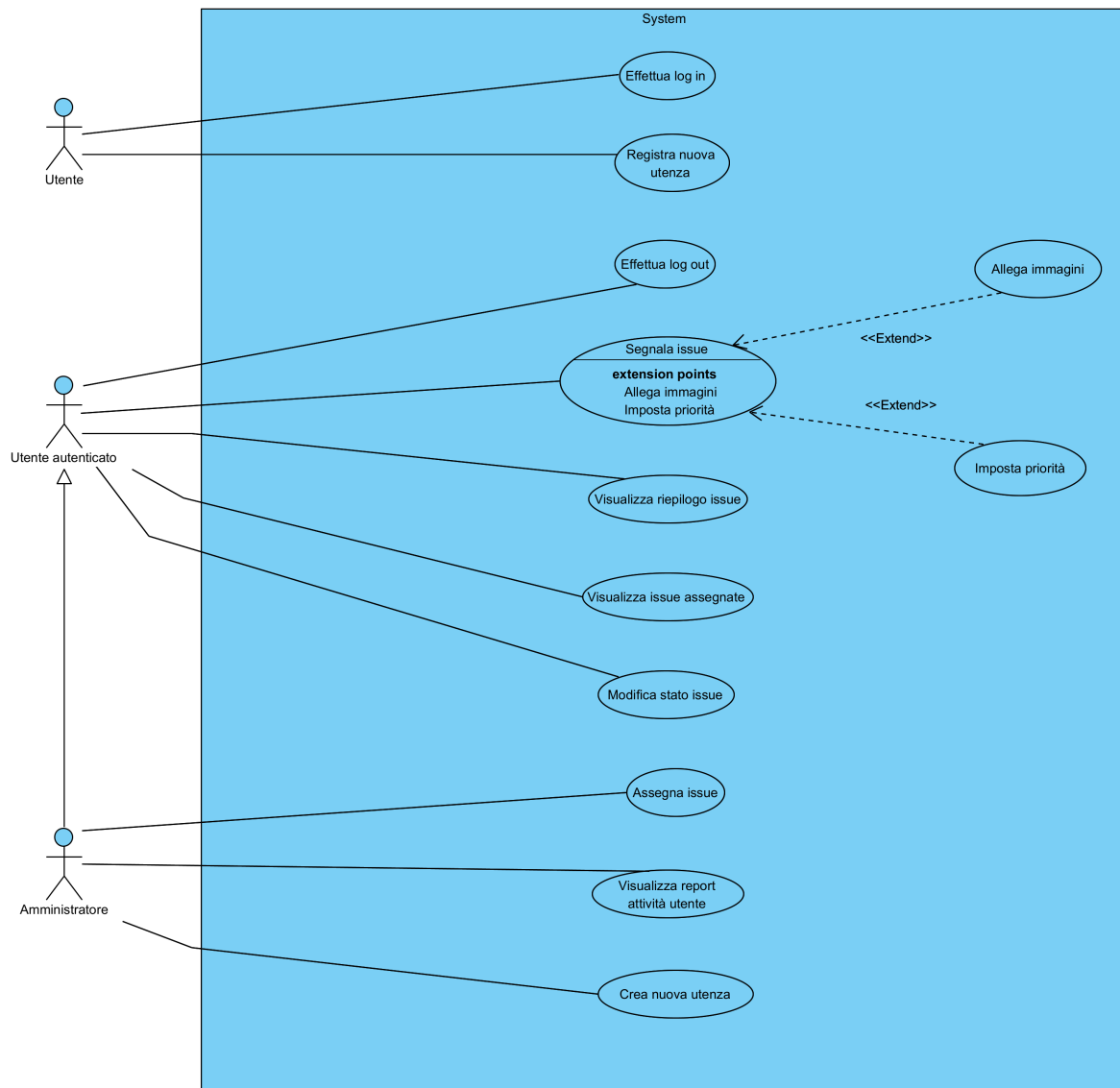
Figura 1: Use Case Diagram
